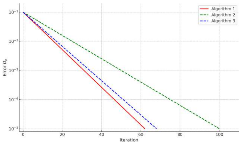
FIGURE 2. Convergence comparison k = 20 and m = 200 .
