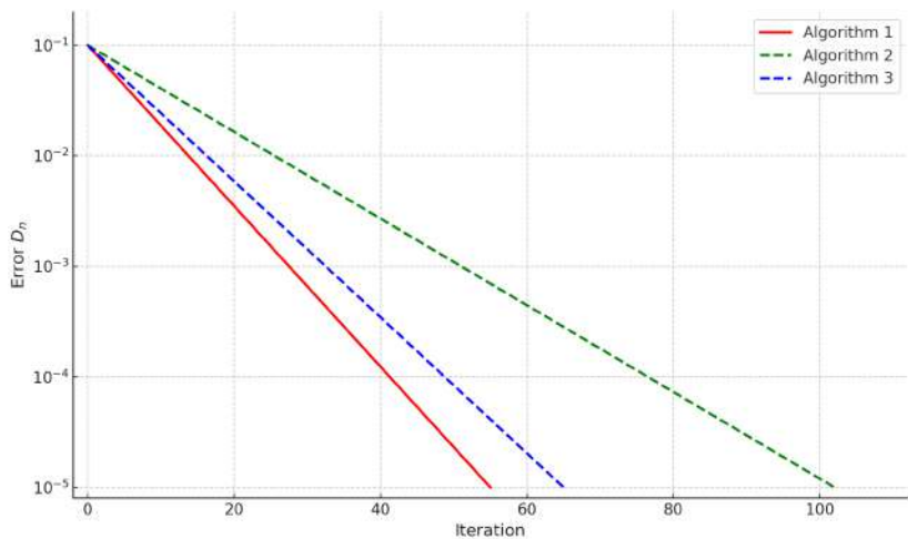
FIGURE 1. Convergence comparison k = 20 and m = 100 .
