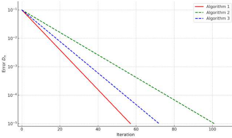
FIGURE 3. Algorithm comparison results.
